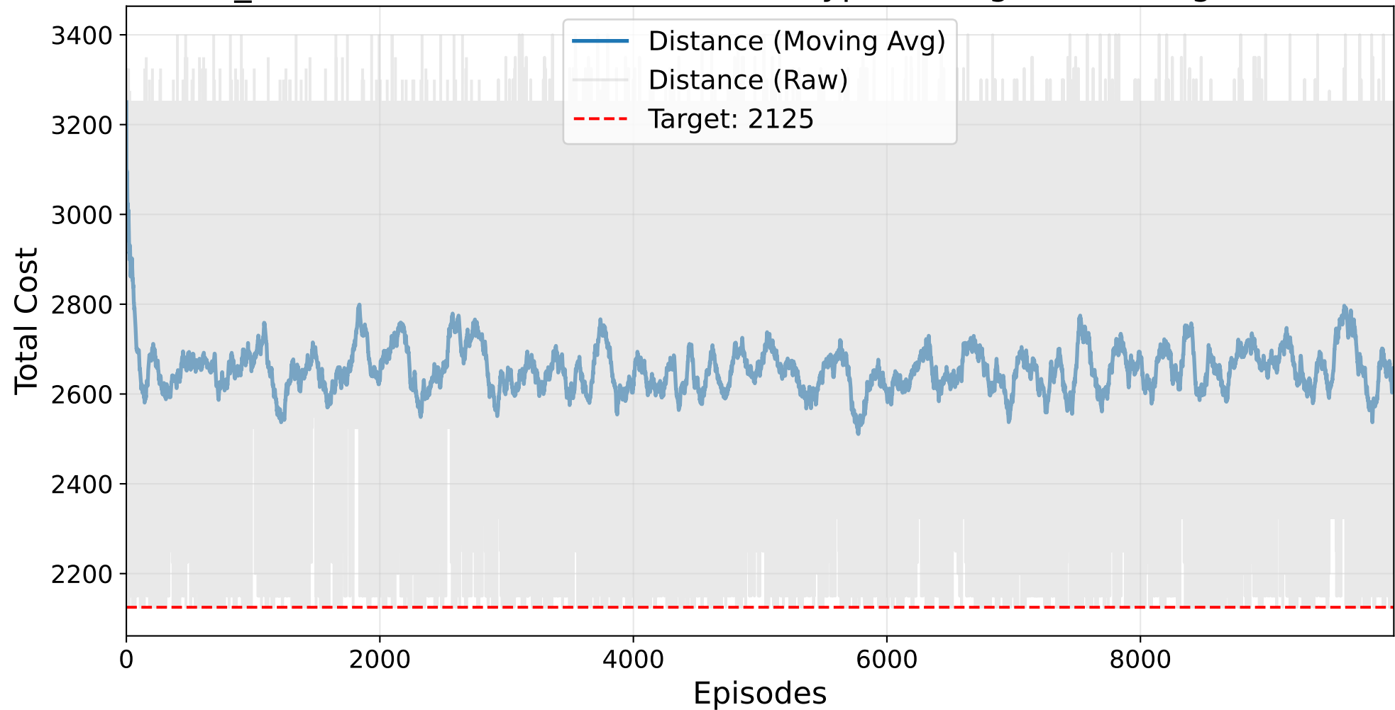
Final NO_BAYESIAN Masked AutoRL-SOP (HyperTuningSK) Training - ESC07.sop
